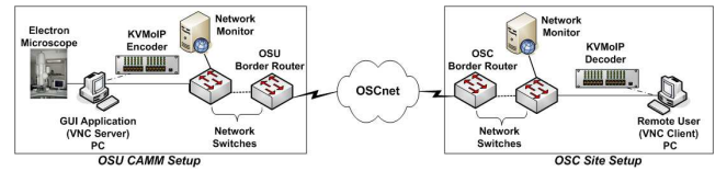
Figure 6: Telemicroscopy testbed setup
