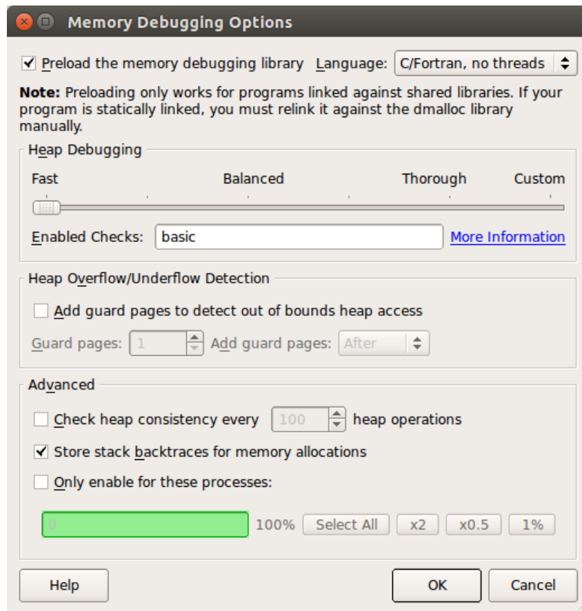
Figure 77: Memory Debugging Options
