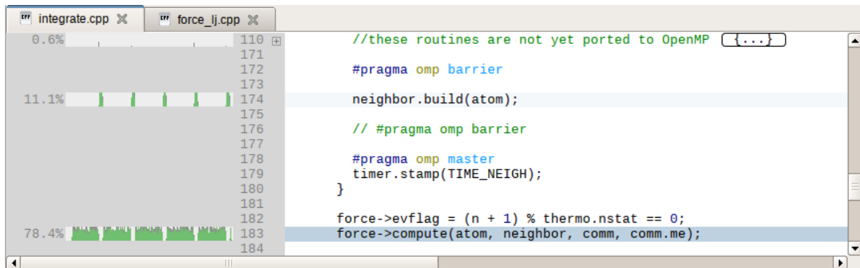
Figure 103: OpenMP Source Code View
