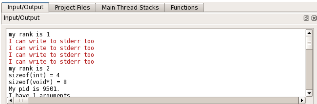
Figure 101: MAP Standard Output Window
