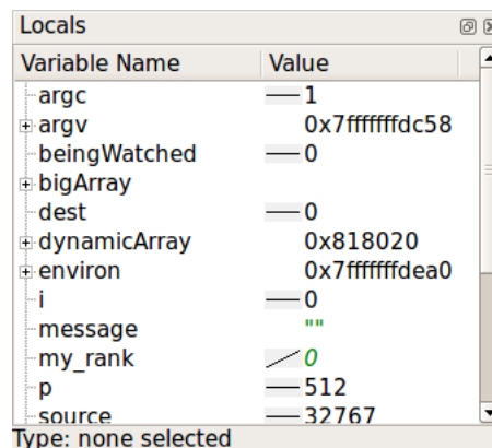
Figure 56: Displaying Variables
