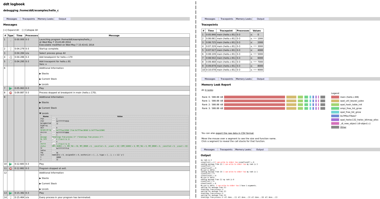
Figure 88: Offline Mode HTML output
