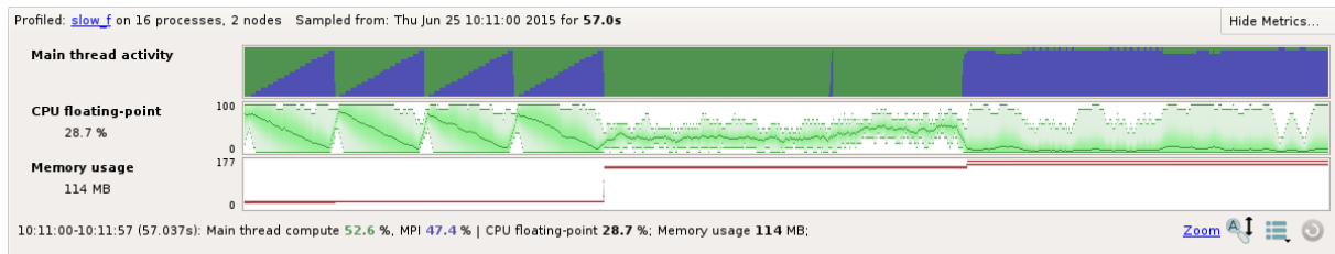
Figure 112: Metrics view
