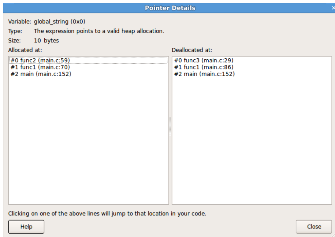
Figure 79: Pointer details
