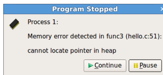
Figure 78: Memory Error Message
