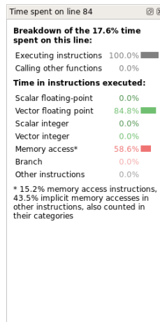
Figure 107: Selected Lines View
