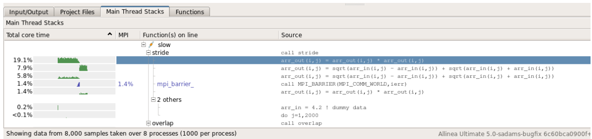
Figure 108: MAP Stacks View
