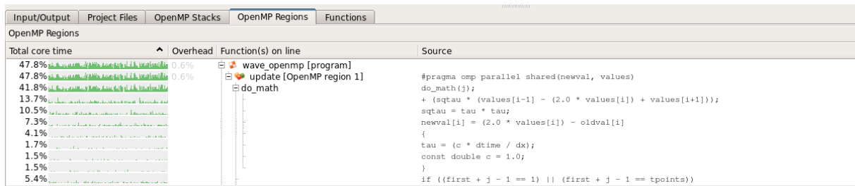
Figure 109: OpenMP Regions View
