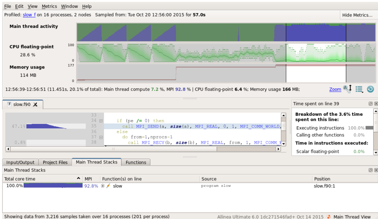
Figure 113: Map with a region of time selected
