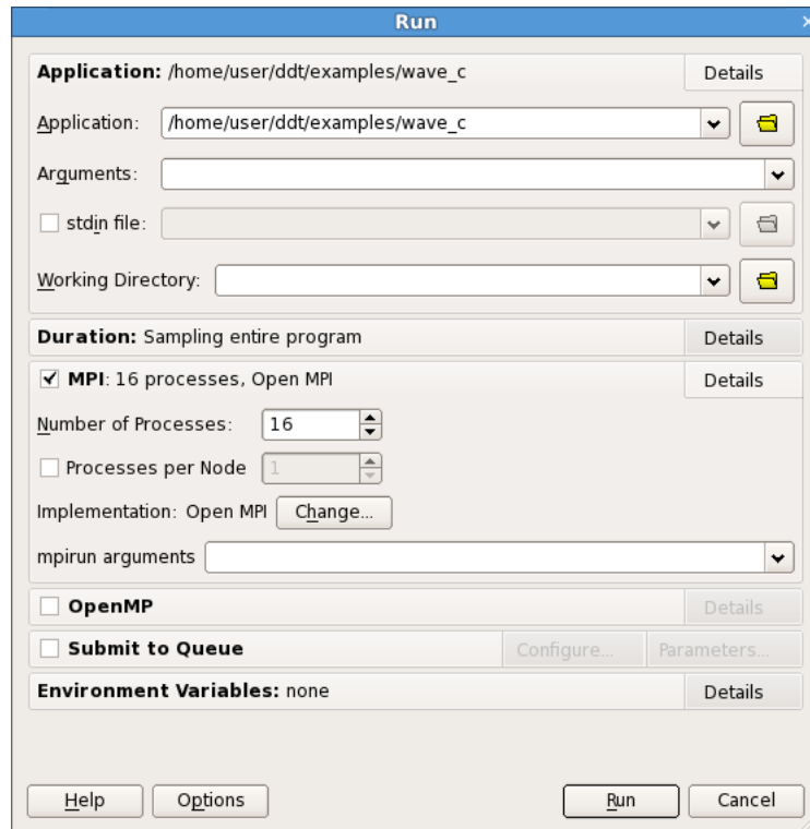
Figure 95: Run window
