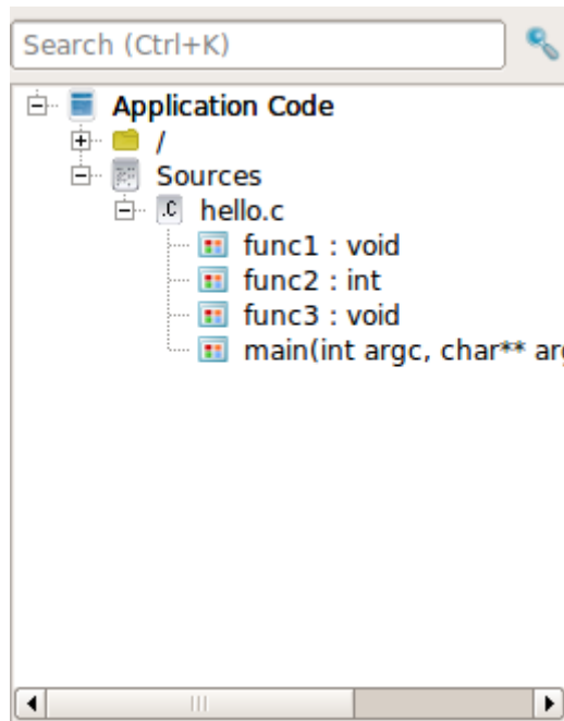
Figure 29: Function Listing
