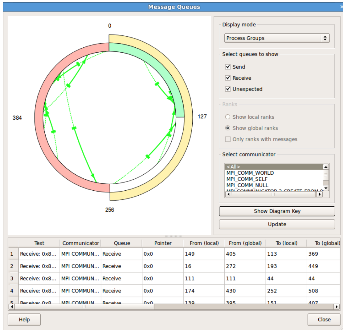
Figure 76: Message Queue Window
