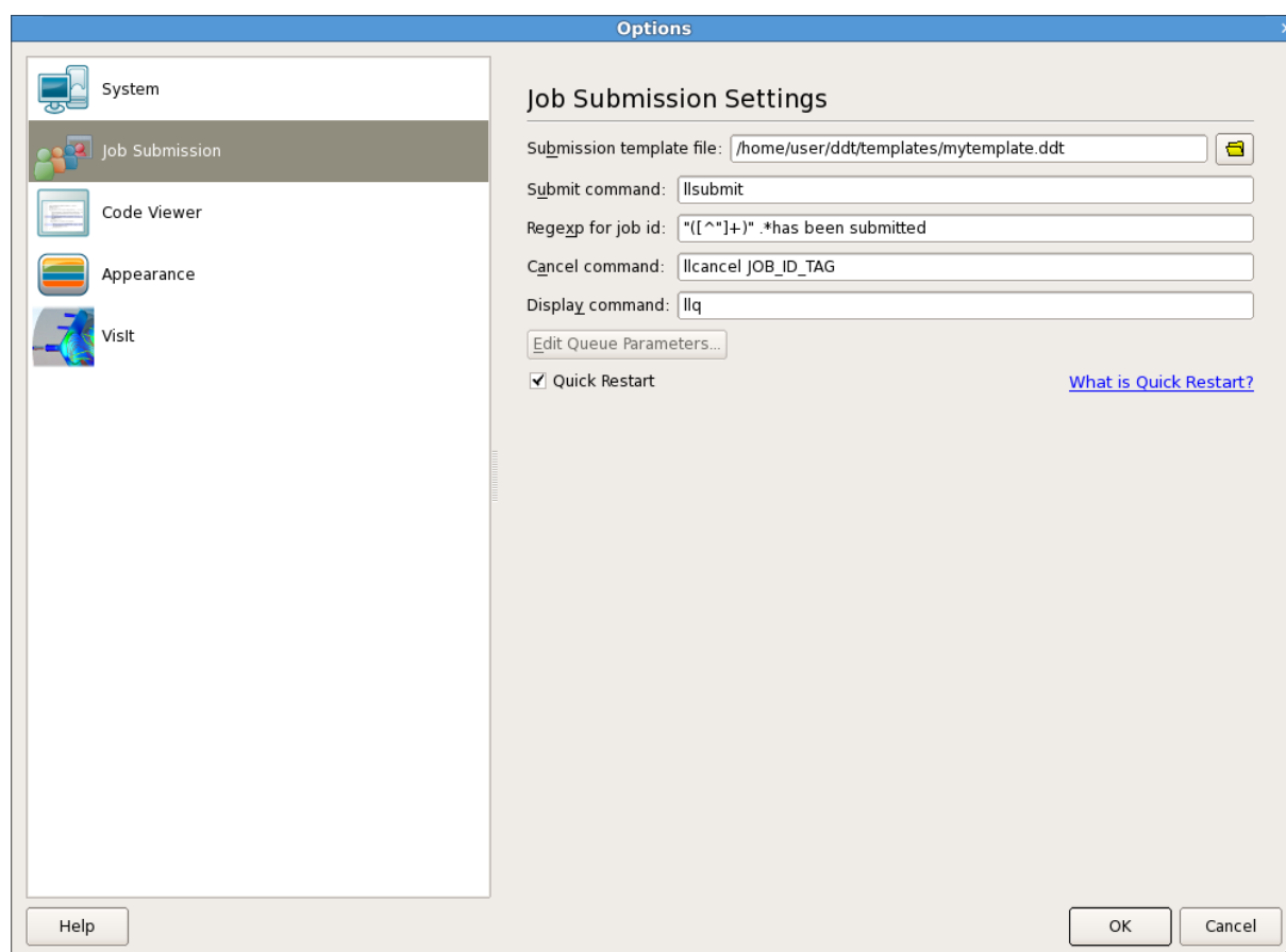
Figure 115: Queuing Systems
