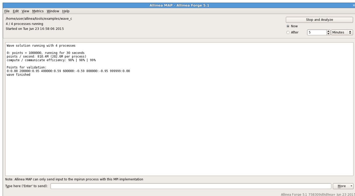
Figure 96: Running window
