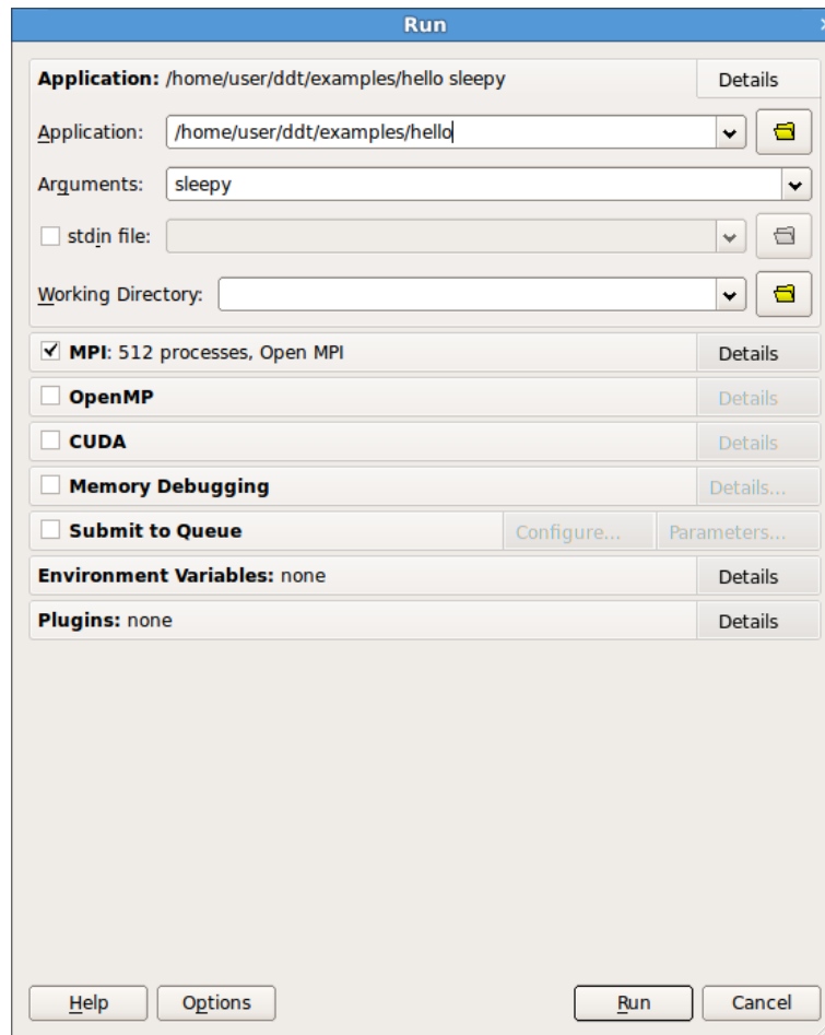
Figure 12: Run Window
