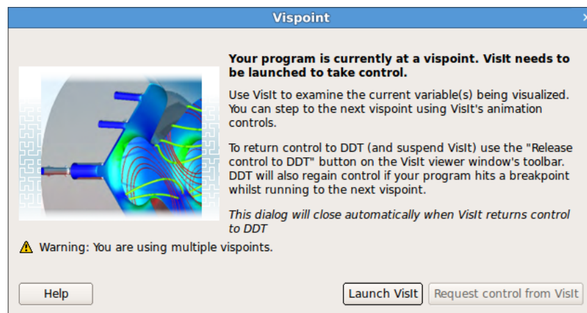
Figure 91: Vispoint window
