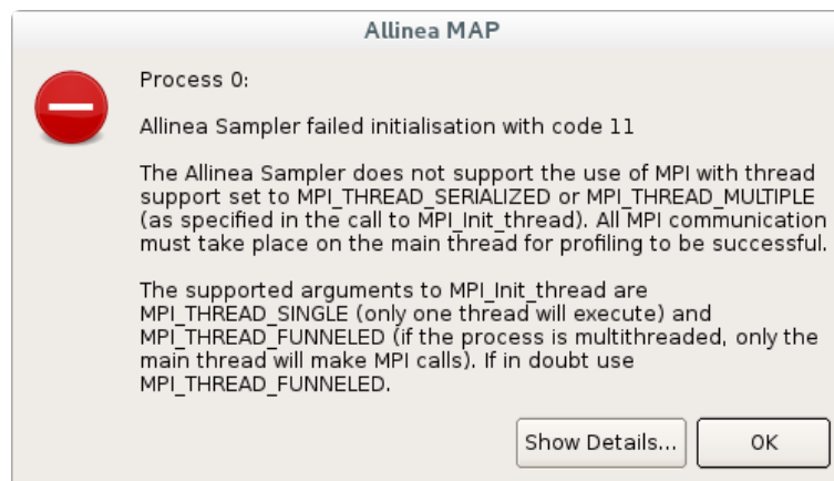
Figure 116: Restricted thread support error
