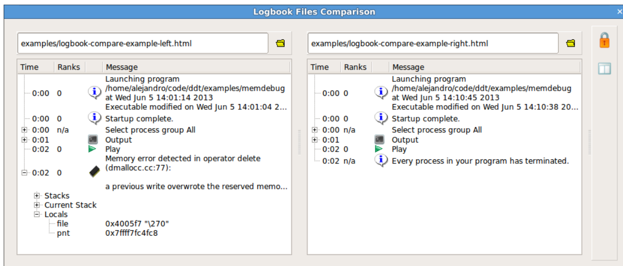
Figure 75: Logbook comparison window with tracepoint difference selected
