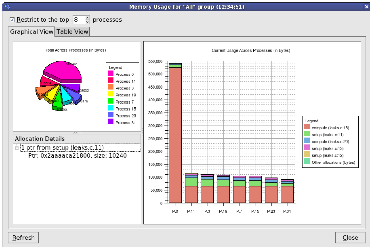
Figure 81: Memory Usage Graphs
