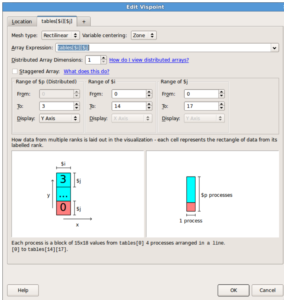
Figure 90: Add/edit vispoint window
