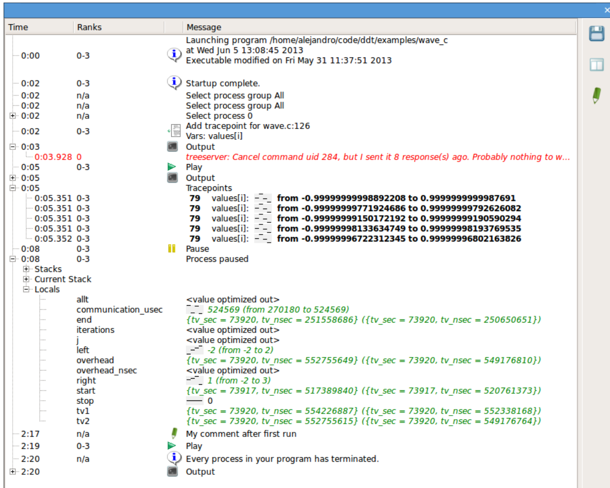
Figure 74: Logbook example of a debug session
