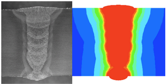
Left: Cross section of real weld
