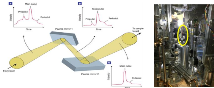
Figure 1: (left) The PM approach to pulse contrast enhancement shown with a double PM system. 41 (right) Photo of experimental chamber configuration for the Astra experiment. A single liquid crystal film device was used, circled in yellow.
